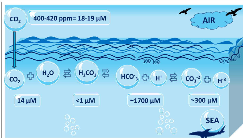
Fig 1. The equilibrium and concentrations of atmospheric- and seawater-CO 2 . Salinity and temperature make the equilibrated CO 2 level in seawater roughly 20% lower than in air. CO 2 will hydrate to form carbonic acid (H 2 CO 3 ), which dissociates to bicarbonate (HCO 3 - ) and carbonate (CO 3 2- ). These reactions are pH dependent. The distribution between C chemical forms at an average seawater pH of 8.1 translates in approximately 120 and 20 times higher HCO 3 - and CO 3 2- , respectively, than that of dissolved CO 2 at equilibrium (Beer 2022; Israel & Sphigel 2023).
