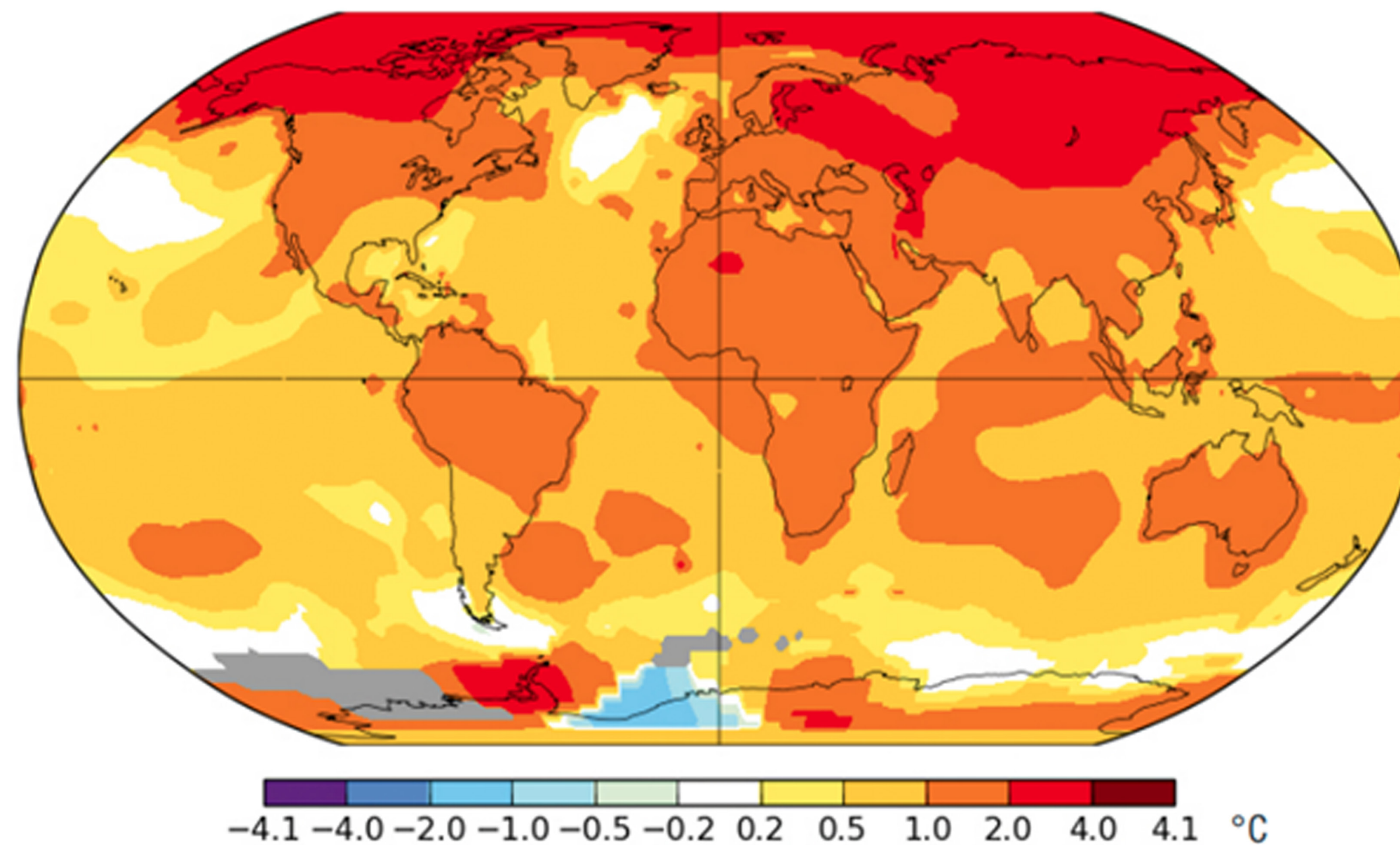
CHANGE IN MEAN ANNUAL SURFACE TEMPERATURE FROM 1950-2018
